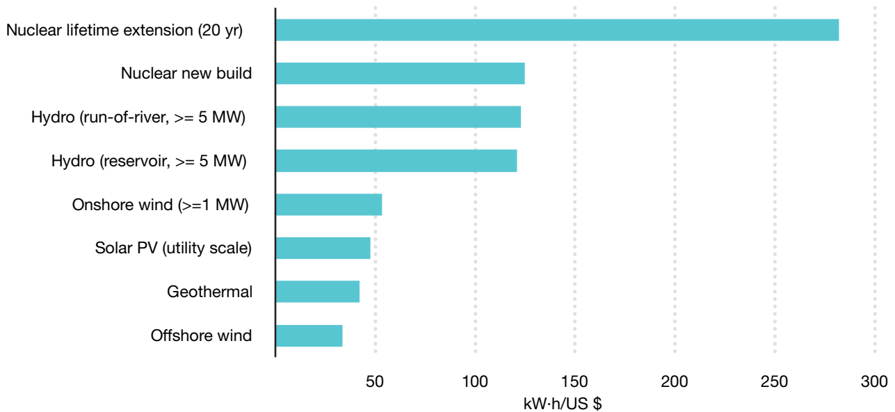
Figure 21. Low carbon electricity generation per unit of investment (median estimates, undiscounted) [44].
